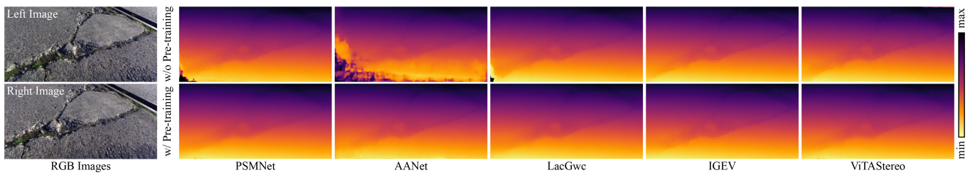
Fig. 7. Depth visualizations for stereo matching on real-world images, comparing models with and without pre-training on synthetic road defect data.
