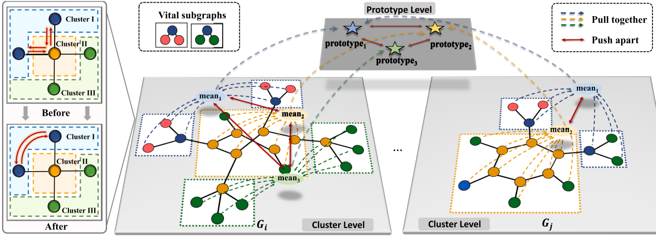
Fig. 3. Illustration of modulating the cluster information flow in CIFlow-GNN at both the cluster level ( \mathcal{L}_{fea} ) and the prototype level ( \mathcal{L}_{proto} ). As a model-level method, the prototypes are shared across clusters within all graphs.
