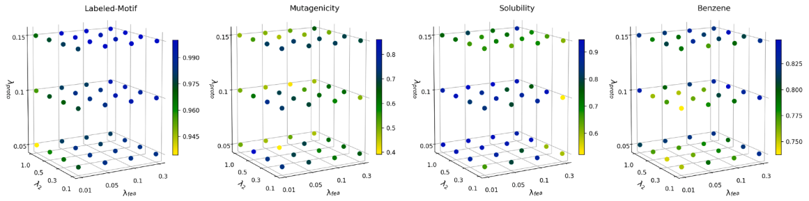
(c) Interpretation performance with respect to the parameter \lambda_2 , \lambda_{\text{fea}} , and \lambda_{\text{proto}} on 4 datasets
