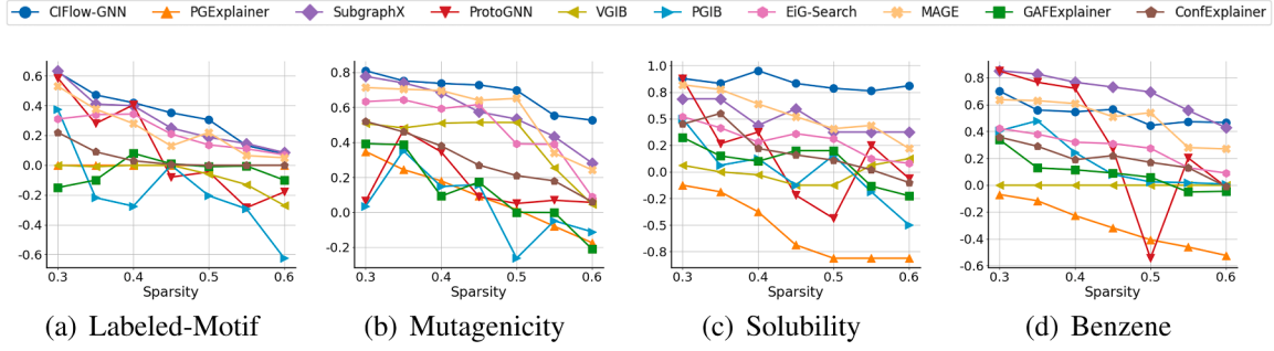
Fig. 5. Comparisons of fidelity scores ( F \uparrow ) across different sparsity levels. PGExplainer, EiG-Search, and GAFExplainer are edge-based methods, whereas others are subgraph-based methods similar to ours. .
