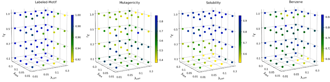
(a) Interpretation performance with respect to the parameters \lambda_2 , \lambda_{\text{con}} , and \lambda_{\text{fea}} on 4 datasets
