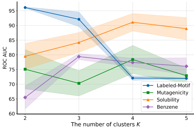
Fig. 7. Interpretation performance (ROC AUC↑) on 4 datasets ( C = 2 ) across different cluster numbers ( K = 2, 3, 4 ) over 3 experiments.
