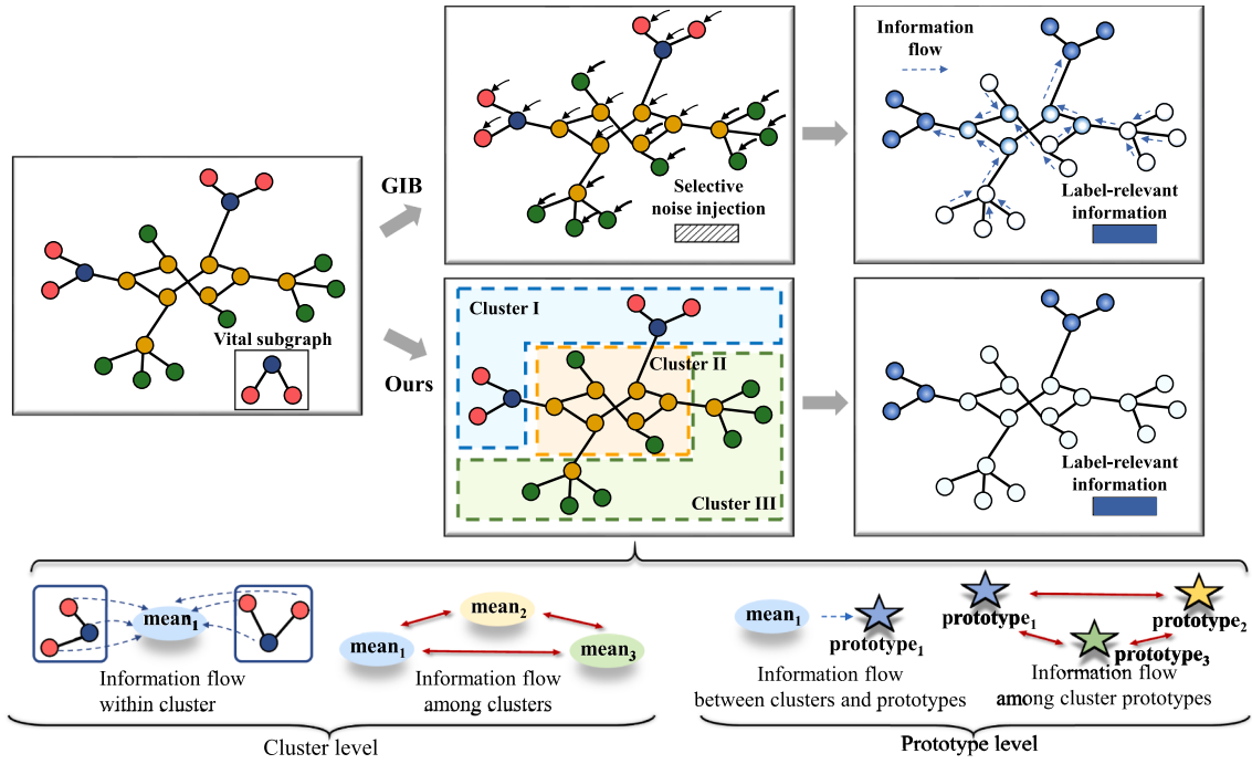
Fig. 1. Comparison of the information flow of GIB methods and the cluster information flow of CIFlow-GNN. The GIB methods employ a selective noise injection method to modulate the label-relevant information flow among nodes from the input graph to the predicted subgraphs. In contrast, our method modulates cluster information flow by identifying clusters and adjusting inter-/intra-cluster interactions at both the cluster and prototype levels. .
