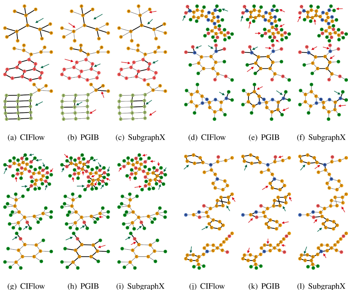
Fig. 9. Visualization of label-relevant subgraphs on Labeled-Motif (a-c), Mutagenicity (d-f), Solubility (g-i), and Benzene (j-l) datasets. Bold edges connect the nodes that the models consider important. Green arrows mark correctly predicted subgraphs, while red arrows highlight incorrect predictions, including both missed important subgraphs and falsely identified unimportant subgraphs. (For interpretation of the references to colour in this figure legend, the reader is referred to the web version of this article.)
