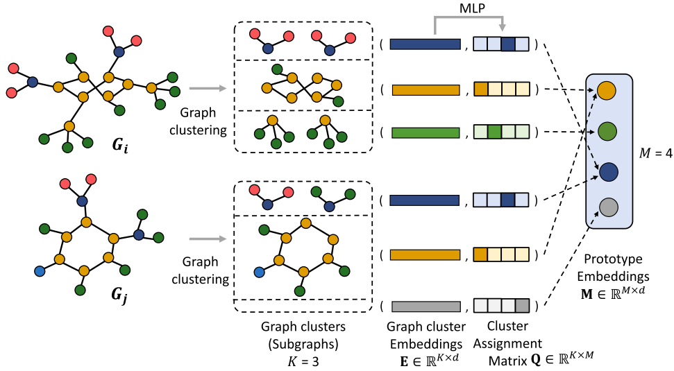
Fig. 4. Illustration of the prototype embeddings computation process.
