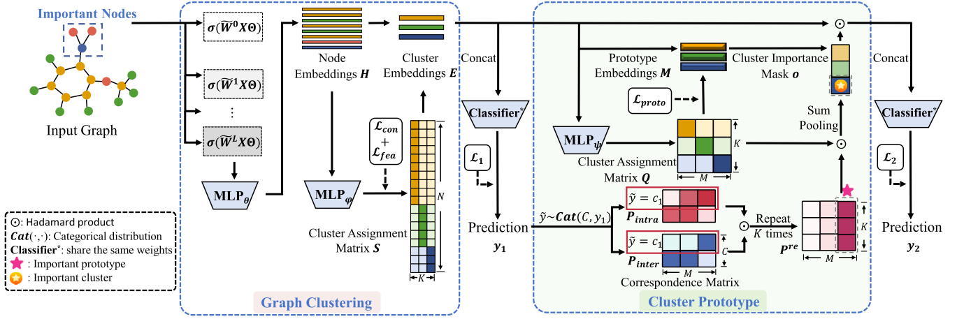
Fig. 2. Overview of the proposed CFlow-GNN framework.
