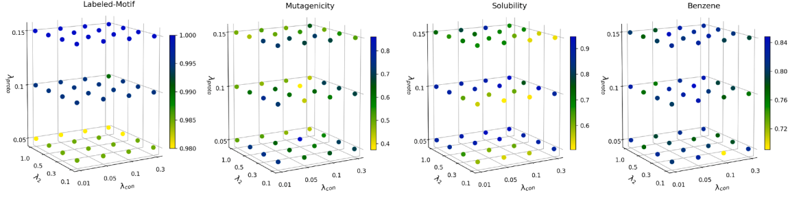
(b) Interpretation performance with respect to the parameter \lambda_2 , \lambda_{\text{con}} , and \lambda_{\text{proto}} on 4 datasets
