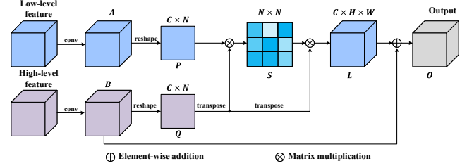
Fig. 2. Our proposed Multi-Scale Feature Fusion Module.
